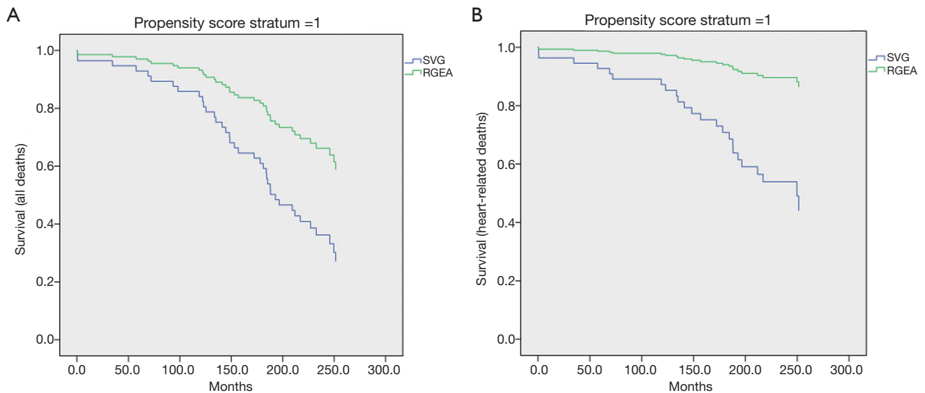
Figure 1 The Kaplan-Meier curves for lowest quintile of the propensity score in the BITA/RGEA vs. BITA/SVG comparison. A. Overall survival; B. Cardiac death
